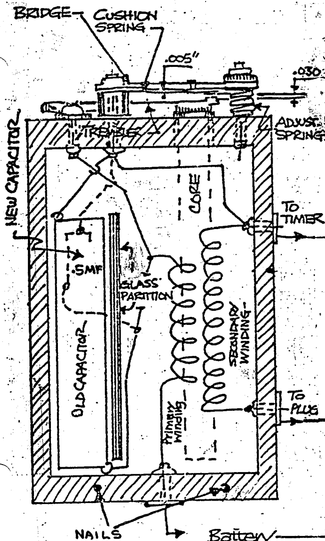
COIL UNIT DETAIL (Partially schematic)
